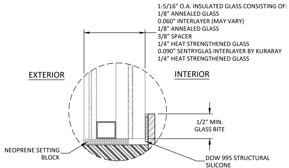
GLAZING DETAIL 3
